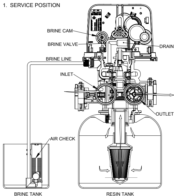
1. SERVICE POSITION
