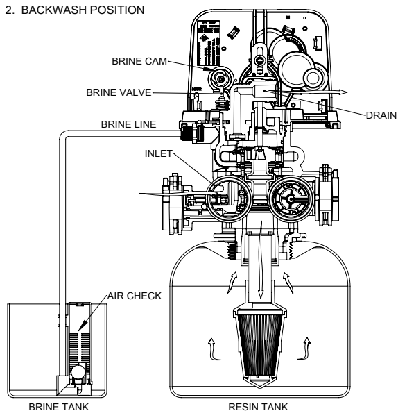
2. BACKWASH POSITION
