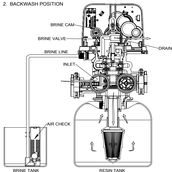
2. BACKWASH POSITION
