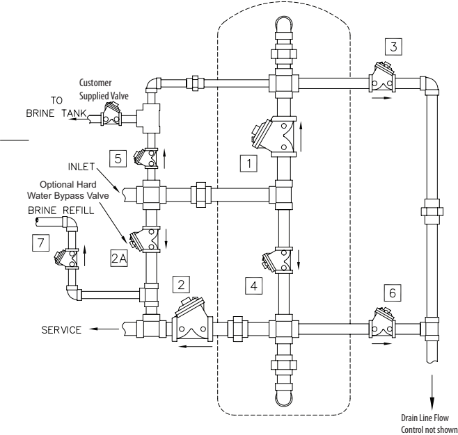
5 POSITION SOFTENER W/ TIMED BRINE REFILL
