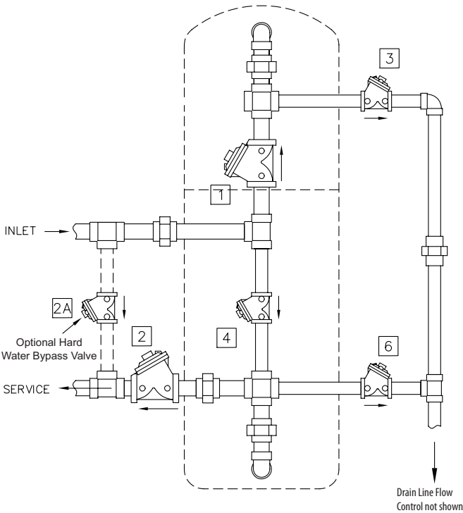
4 POSITION FILTER
